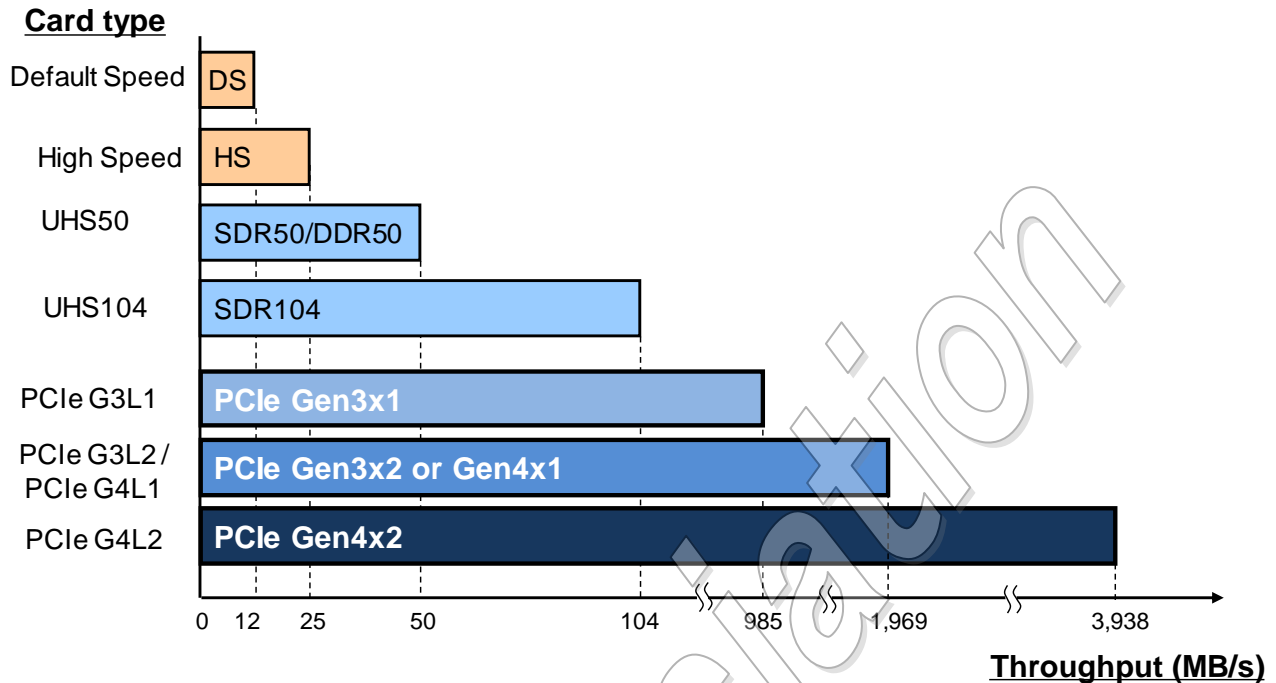
Figure 3-22 : Interface Speed of SD Express Card
