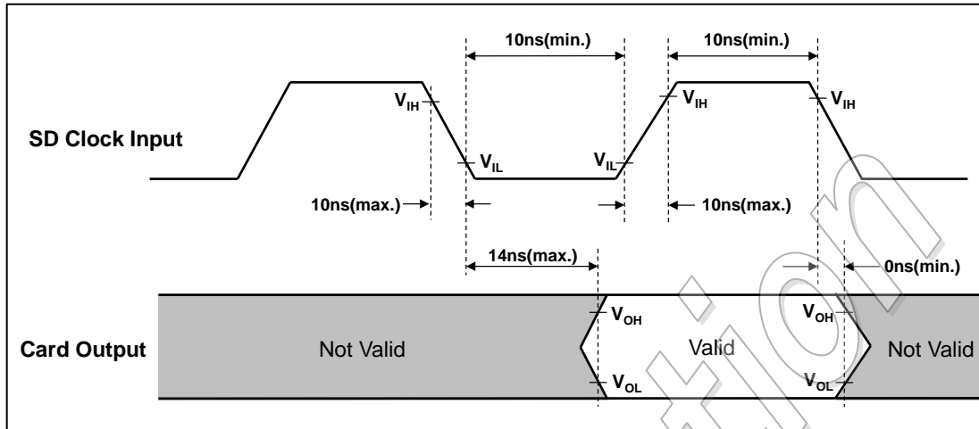
Figure 6-11 : Card Output Timing (Default Speed Mode)
