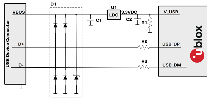
Figure 15: NEO-M9N example circuit for USB interface
