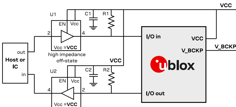
Figure 9: NEO-M9N interface isolation
