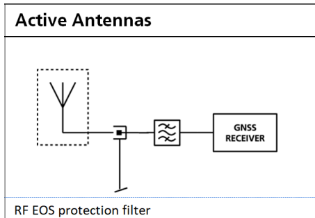
Figure 35: Active antenna EOS protection
