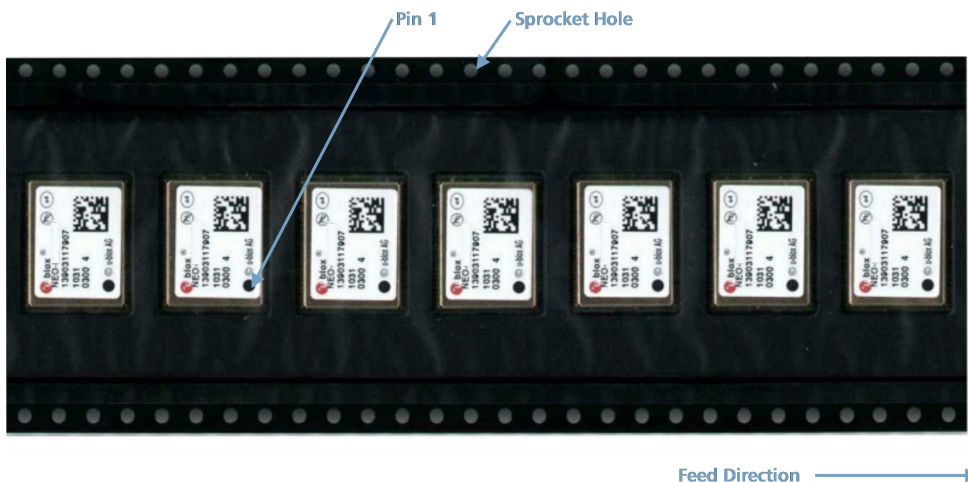
Figure 42: Orientation of NEO-M9N on the tape
