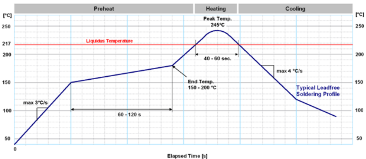
Figure 41: Soldering profile
