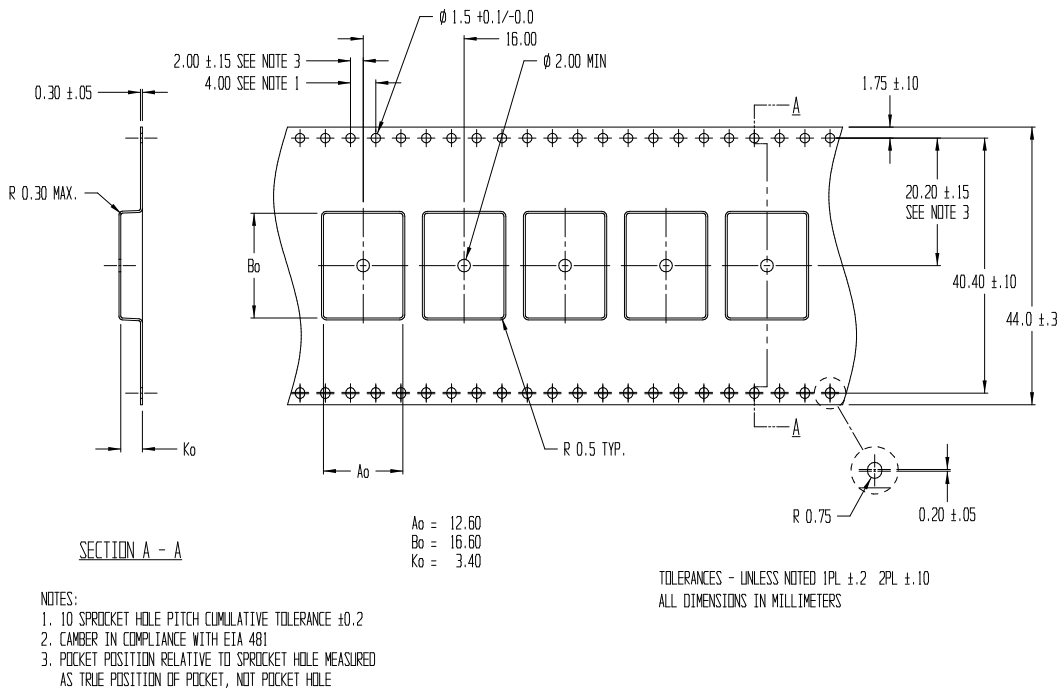
Figure 43: NEO-M9N tape dimensions (mm)
