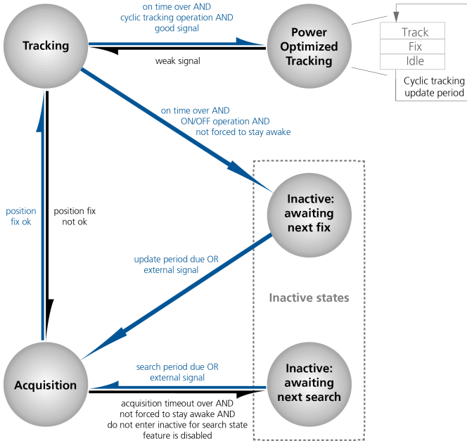
Figure 18: State machine
