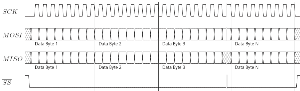
Figure 14: SPI back-to-back read/write access
