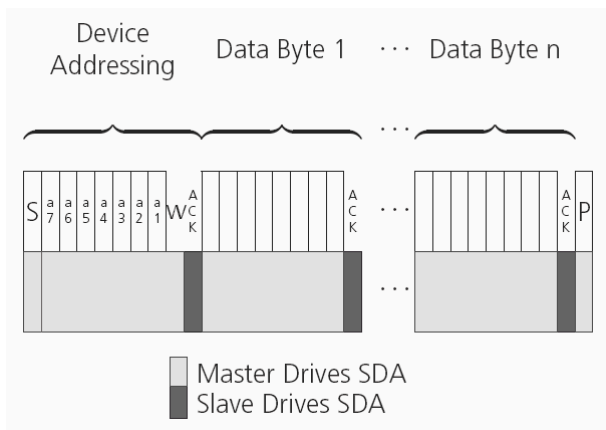
Figure 13: I2C write access
