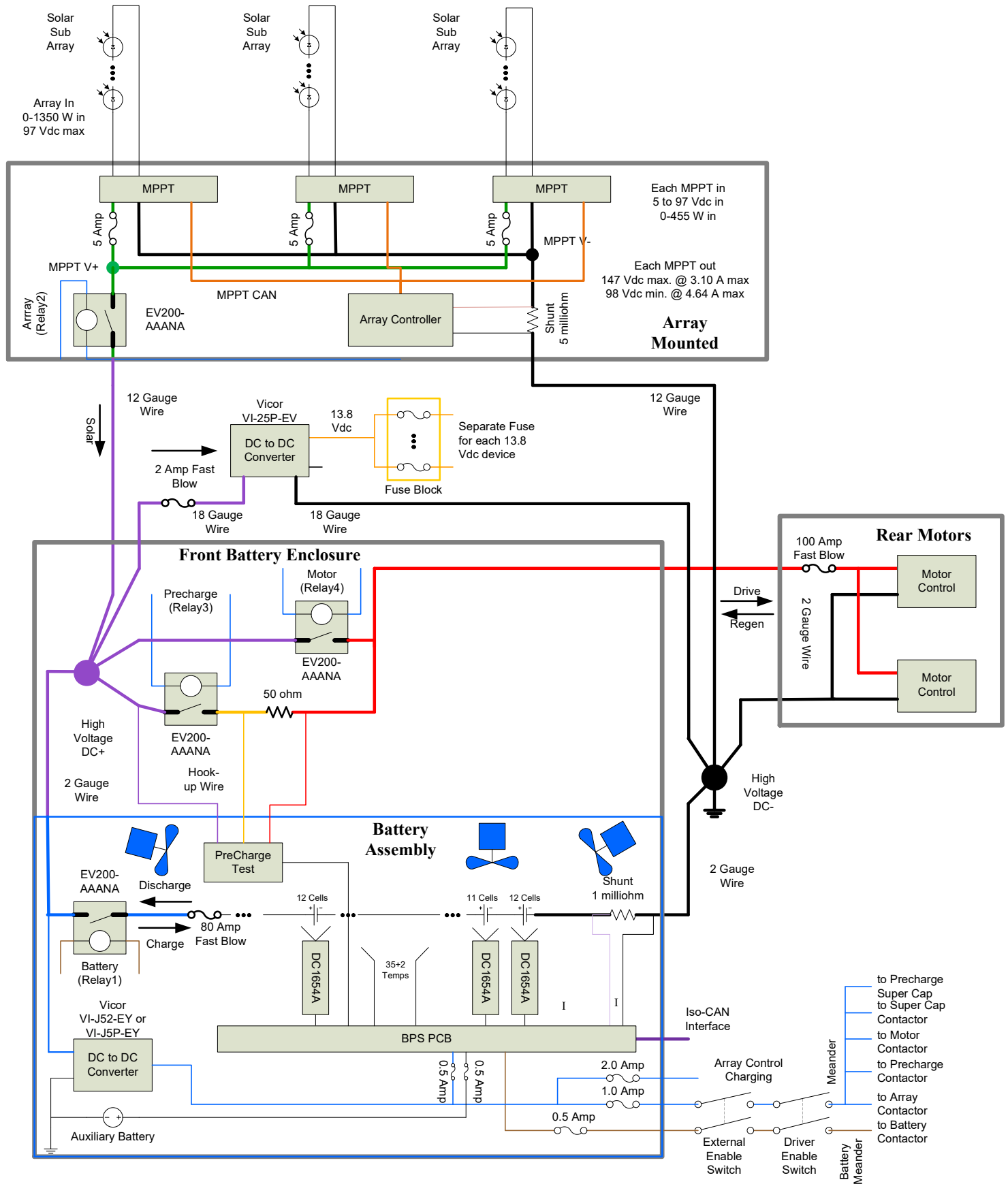
WMU Sunseeker High Power Diagram (Not Complete)
