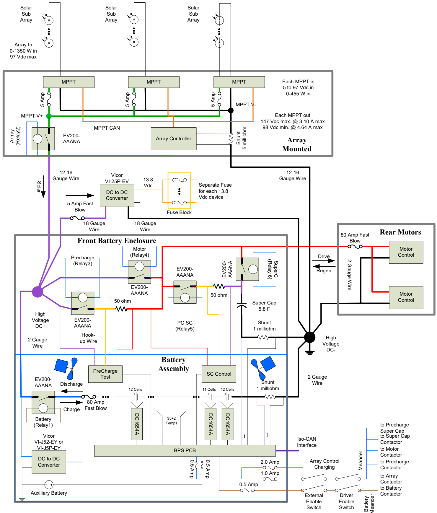
WMU Sunseeker High Power with Super Capacitor Diagram
